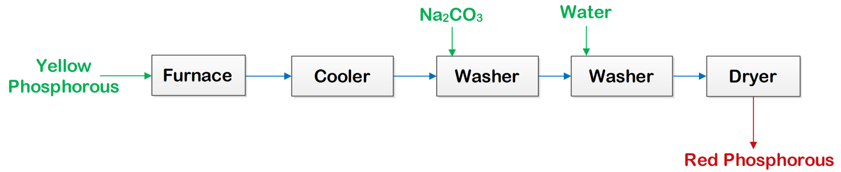
Figure: Manufacturing of Red Phosphorous
